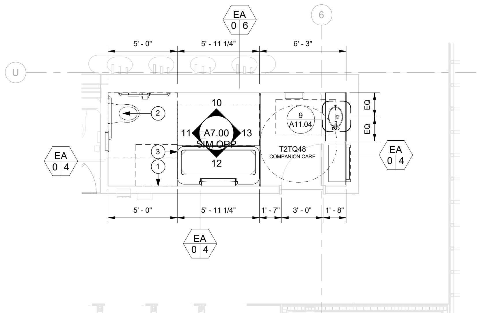
3 TERMINAL - SECTOR E2 - T2TQ48 - ENPLANING - FLOOR PLAN SCALE: 1/4" = 1'-0"
