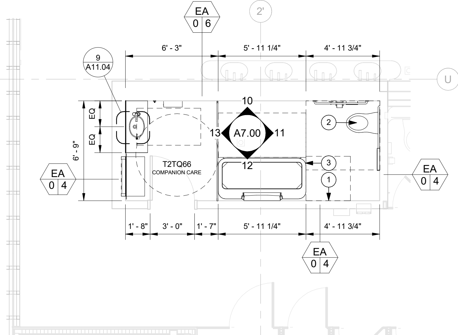
4 TERMINAL - SECTOR 2 - T2TQ66 - ENPLANING - FLOOR PLAN SCALE: 1/4" = 1'-0"
