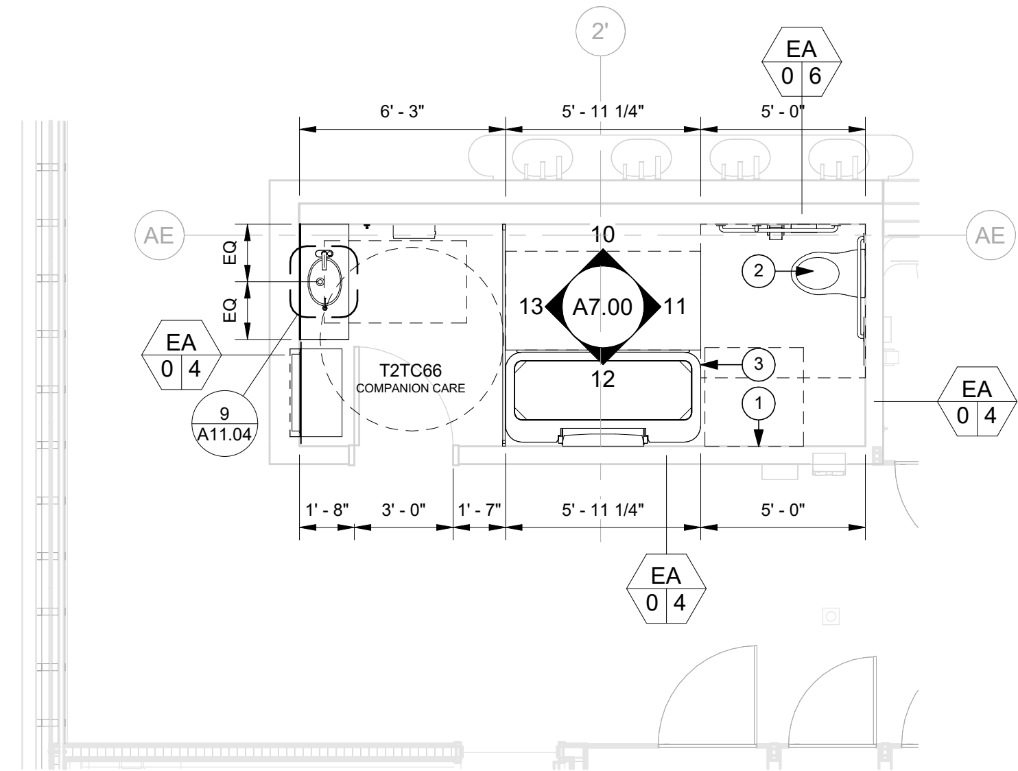
1 TERMINAL - SECTOR W5 - T2TC66 - ENPLANING - FLOOR PLAN SCALE: 1/4" = 1'-0"
