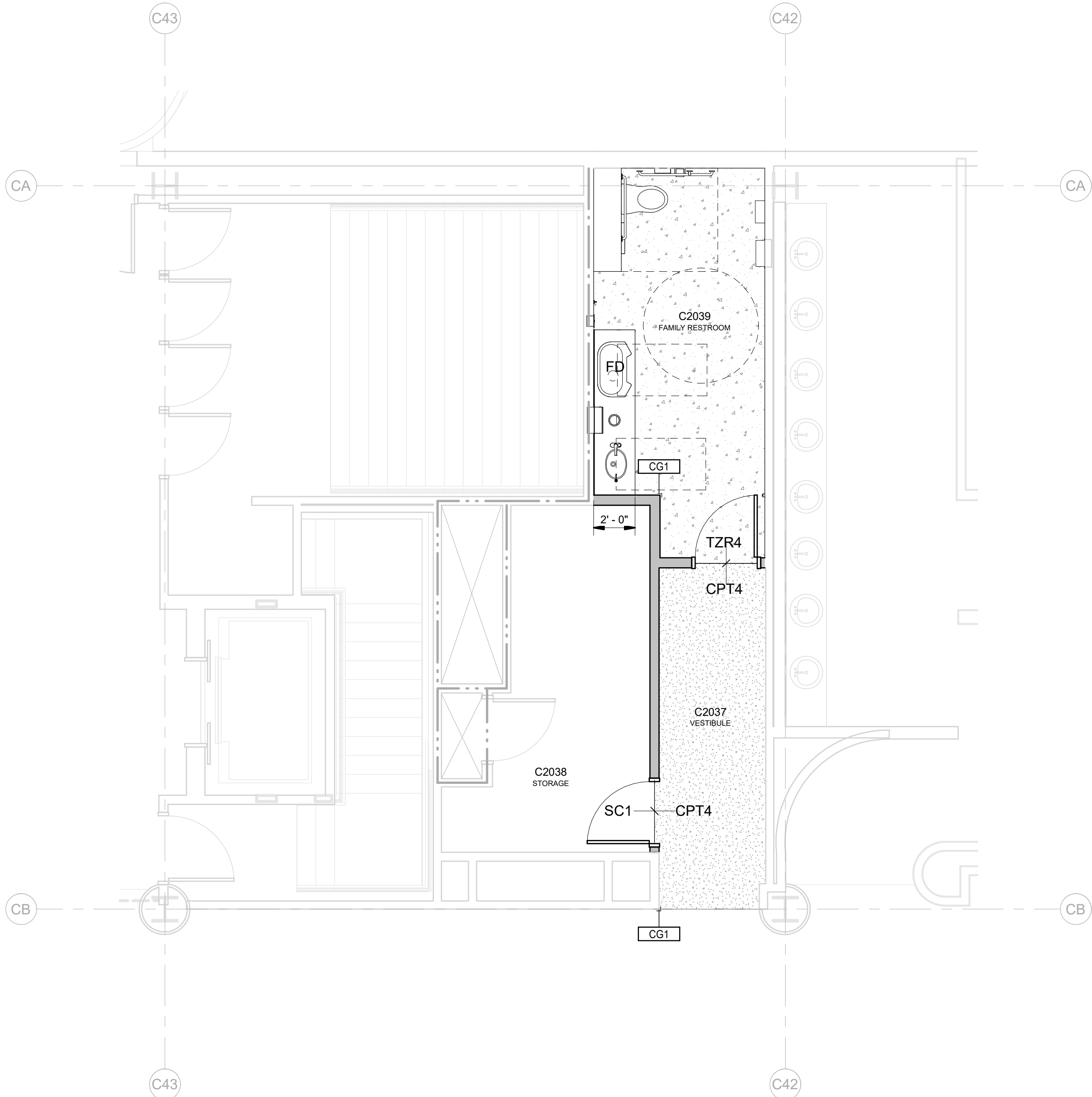
1 CONCURSE C - SECTOR 5 - C2039 - ENPLANING - FINISH PLAN SCALE: 1/4" = 1'-0"
