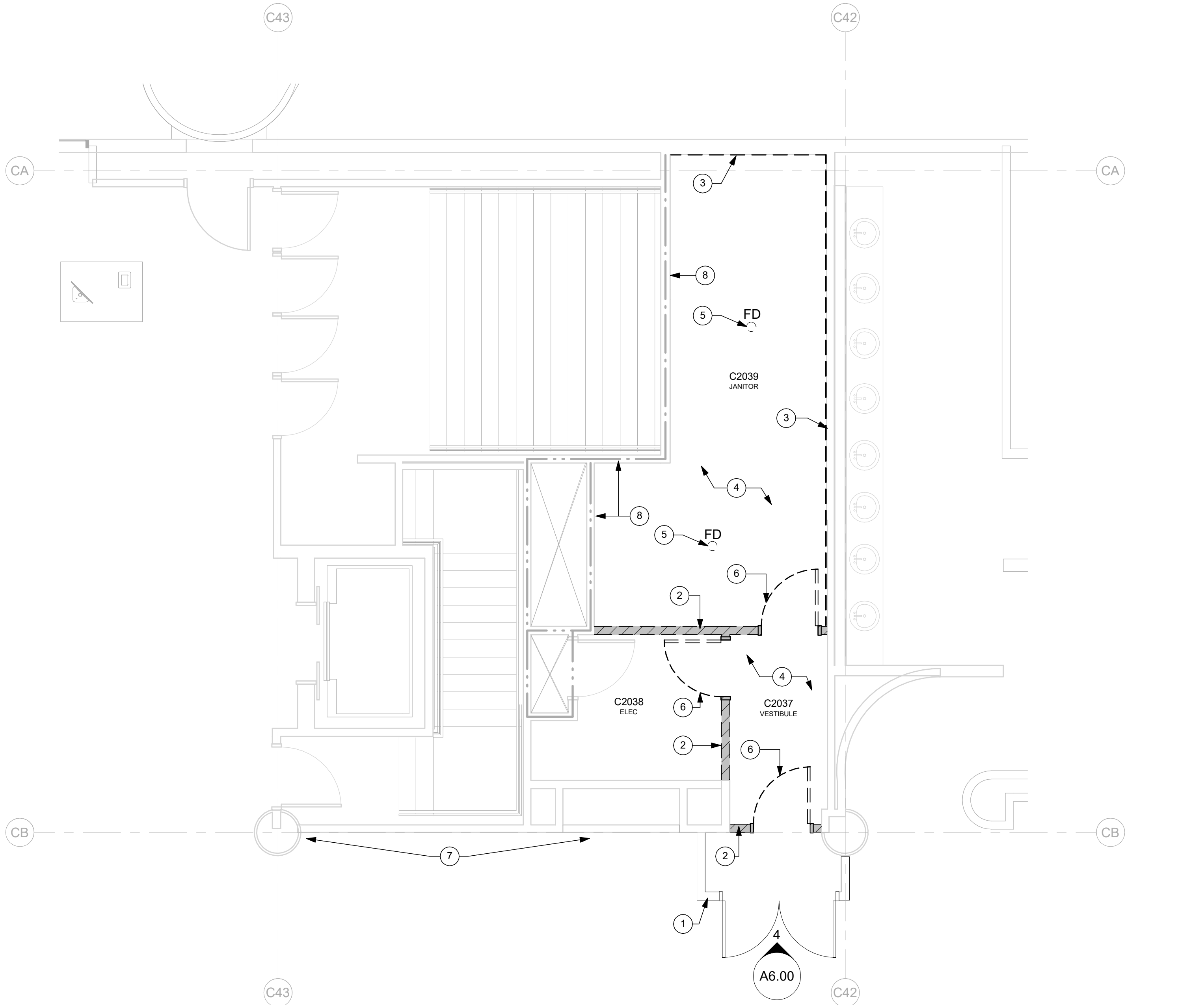
1 CONCURSE C - SECTOR 5 - C2039 - ENPLANING - DEMO PLAN SCALE: 1/4" = 1'-0"
