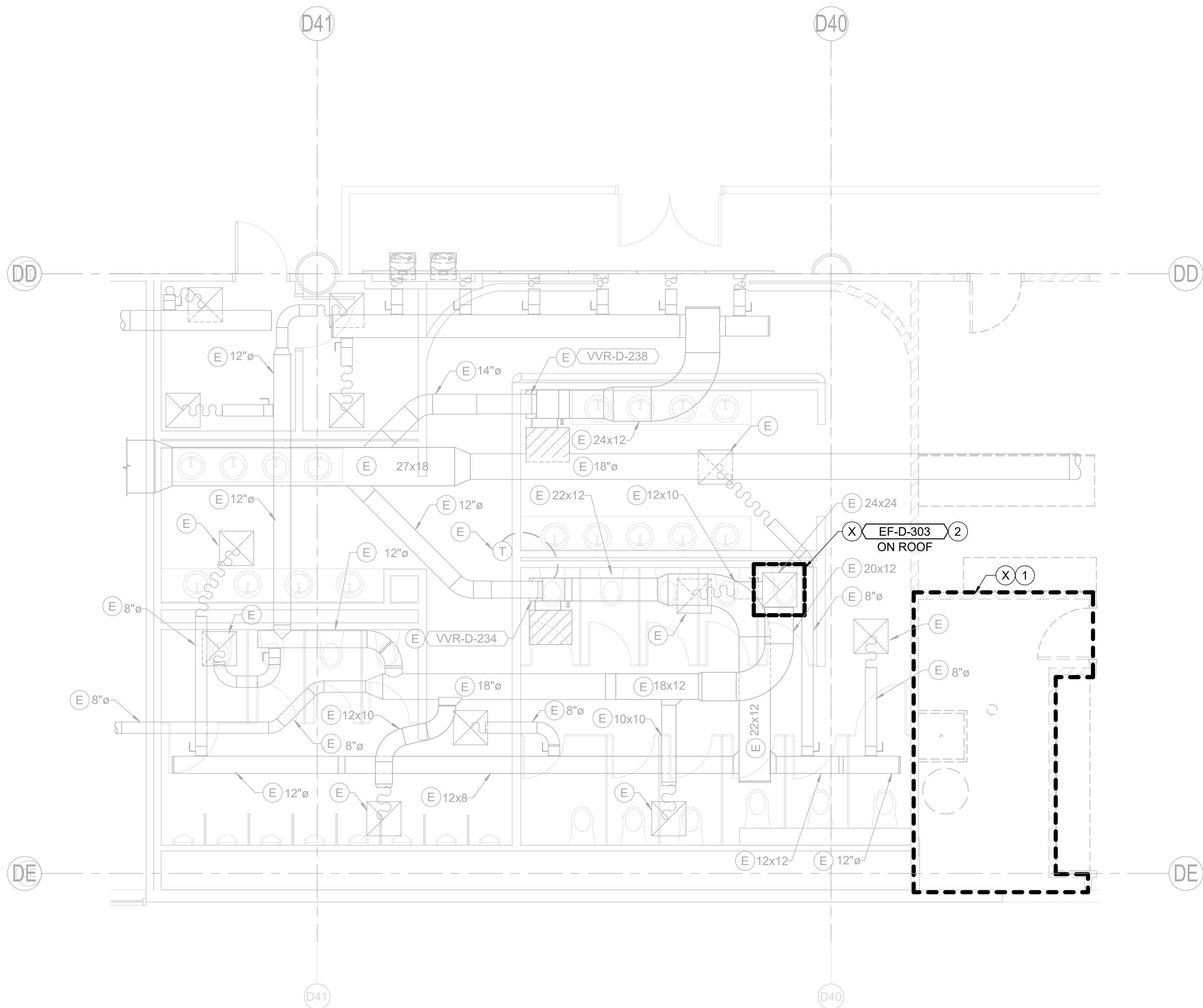
1 CONCURSE D - SECTOR 3 - D2646, D2647 - ENPLANING - DEMO PLAN - MECHANICAL SCALE: 1/4" = 1'-0"
