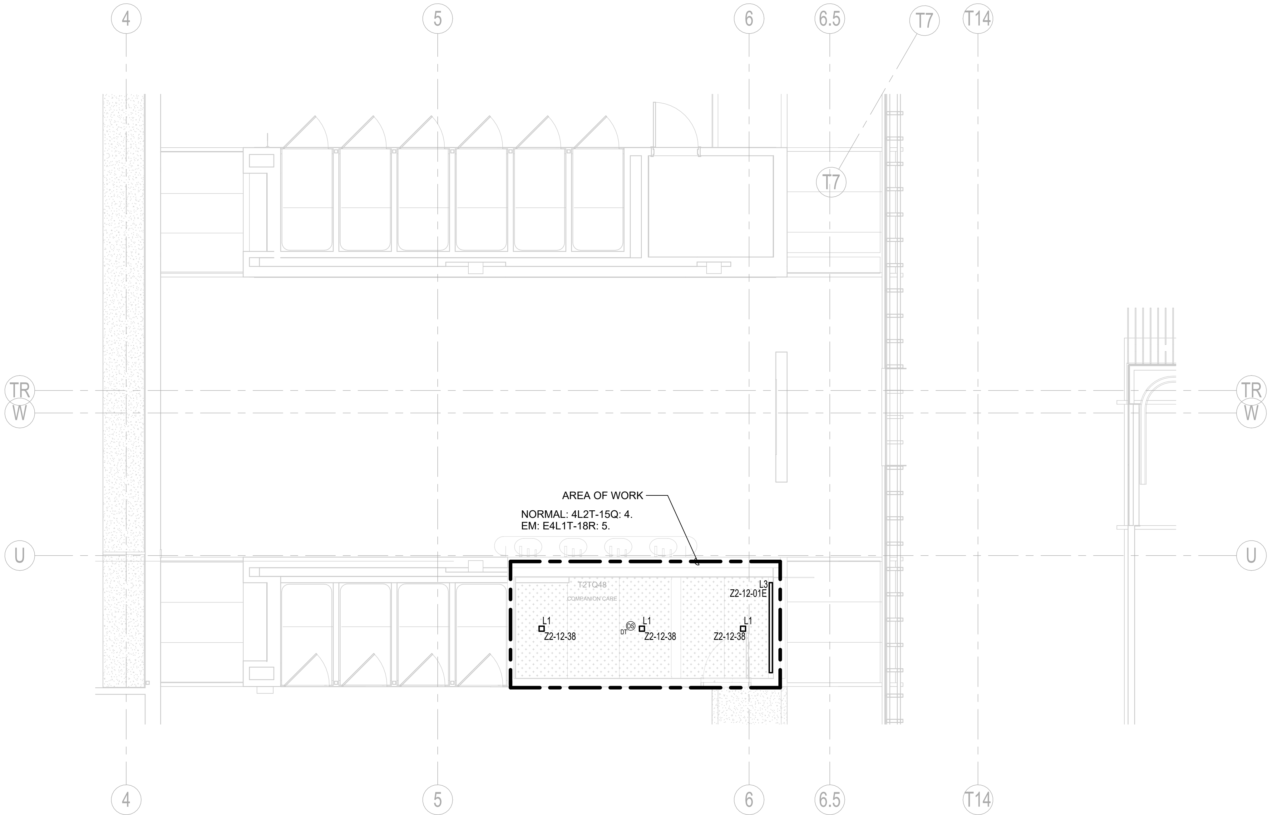
1 TERMINAL - SECTOR E2 - T2TQ48 - ENPLANING - RCP - LIGHTING SCALE: 1/4" = 1'-0"
