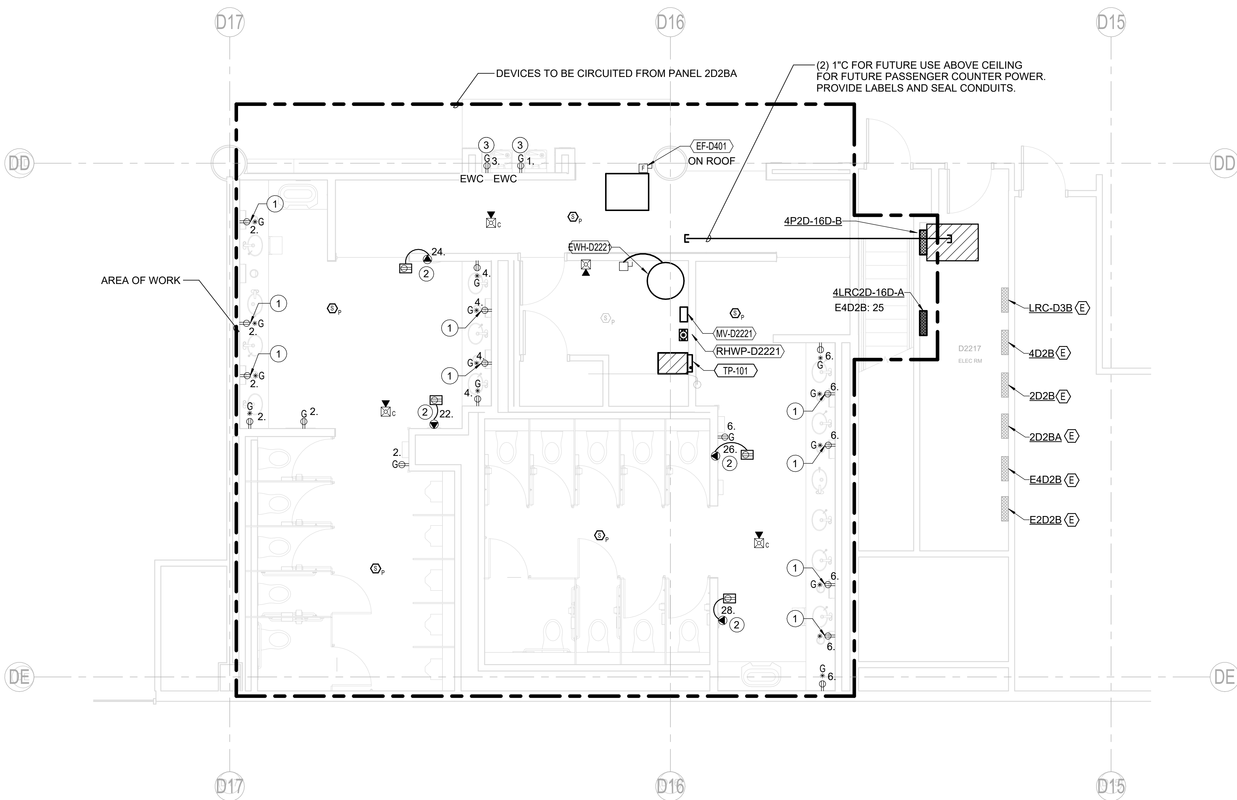
1 CONCURSE D - SECTOR 2 - D2221, D2222, D2223 - ENPLANING - FLOOR PLAN - ELECTRICAL SCALE: 1/4" = 1'-0"
