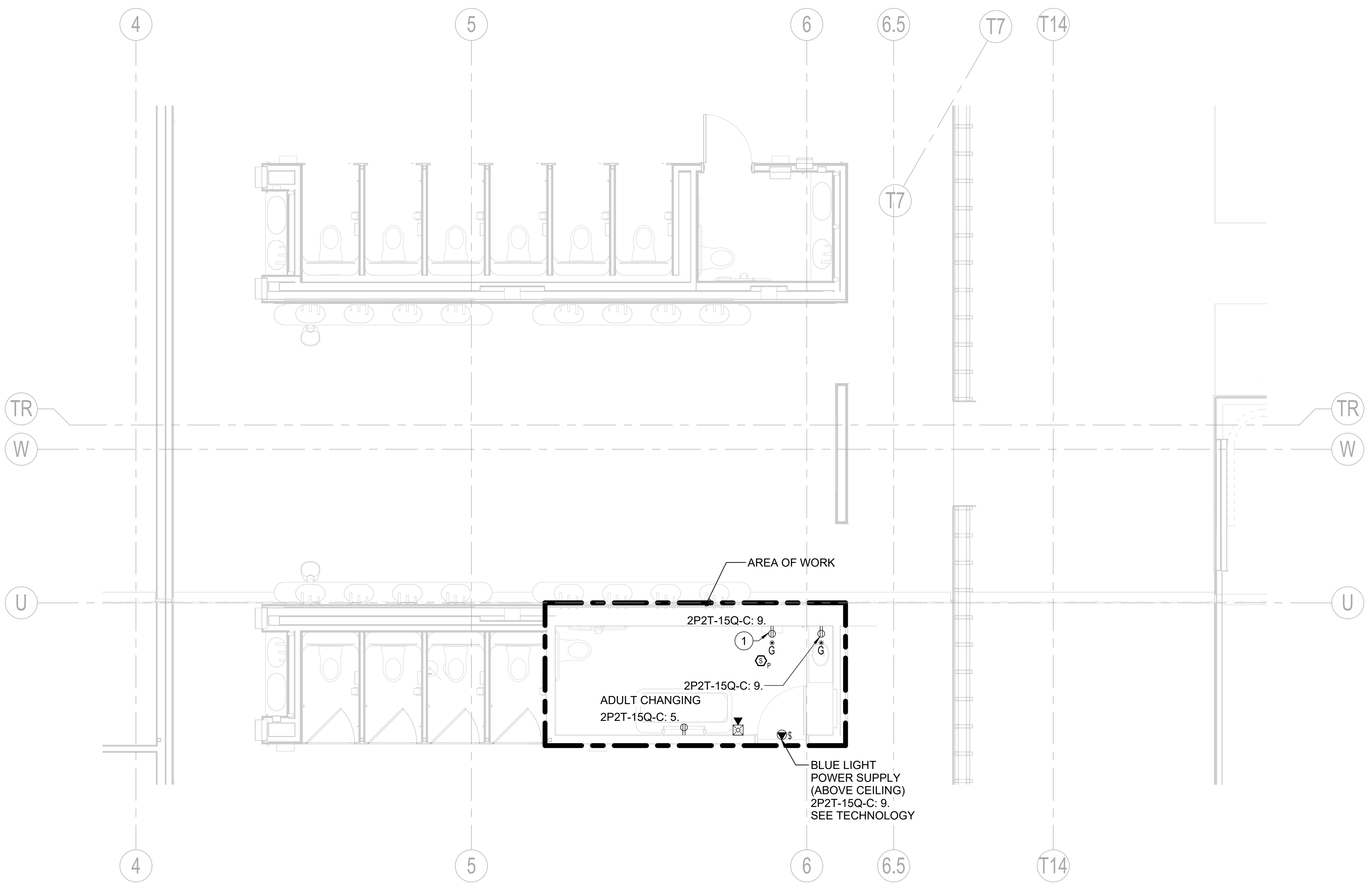
1 TERMINAL - SECTOR E2 - T2TQ48 - ENPLANING - FLOOR PLAN - ELECTRICAL SCALE: 1/4" = 1'-0"
