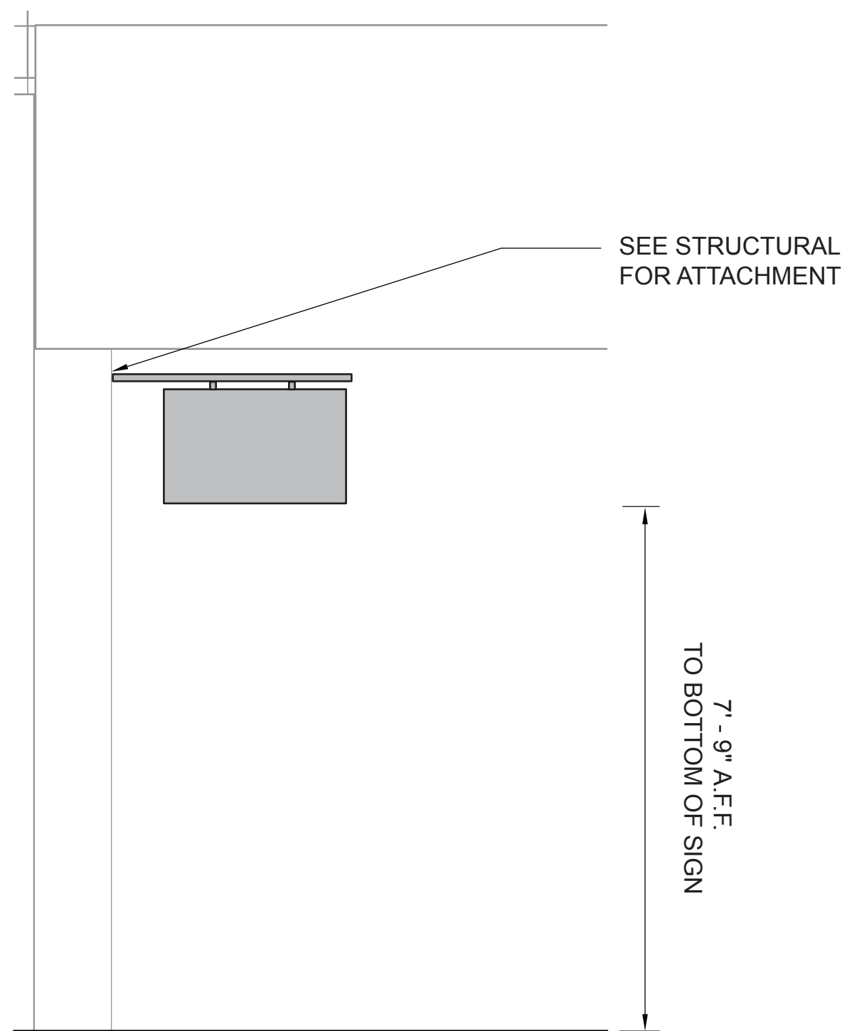
1 CBL - MOUNTING CONDITION SCALE: 1/4" = 1' - 0"
