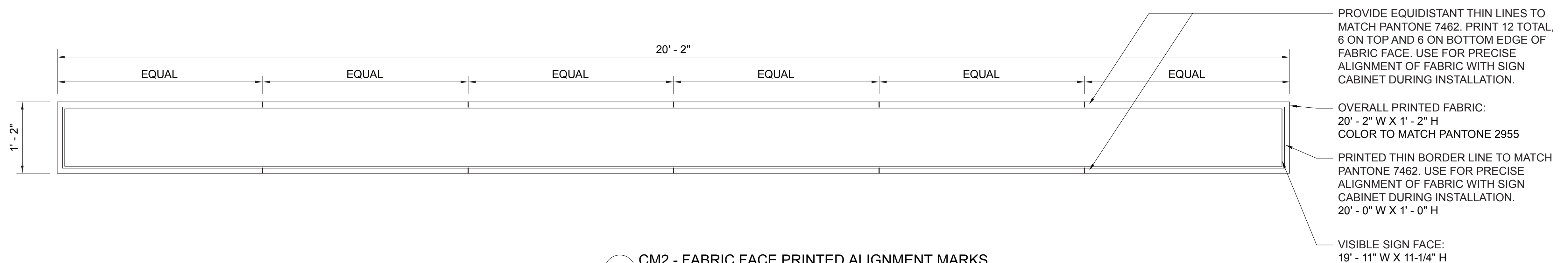
6 CM2 - FABRIC FACE PRINTED ALIGNMENT MARKS SCALE: 1" = 1' - 0"
