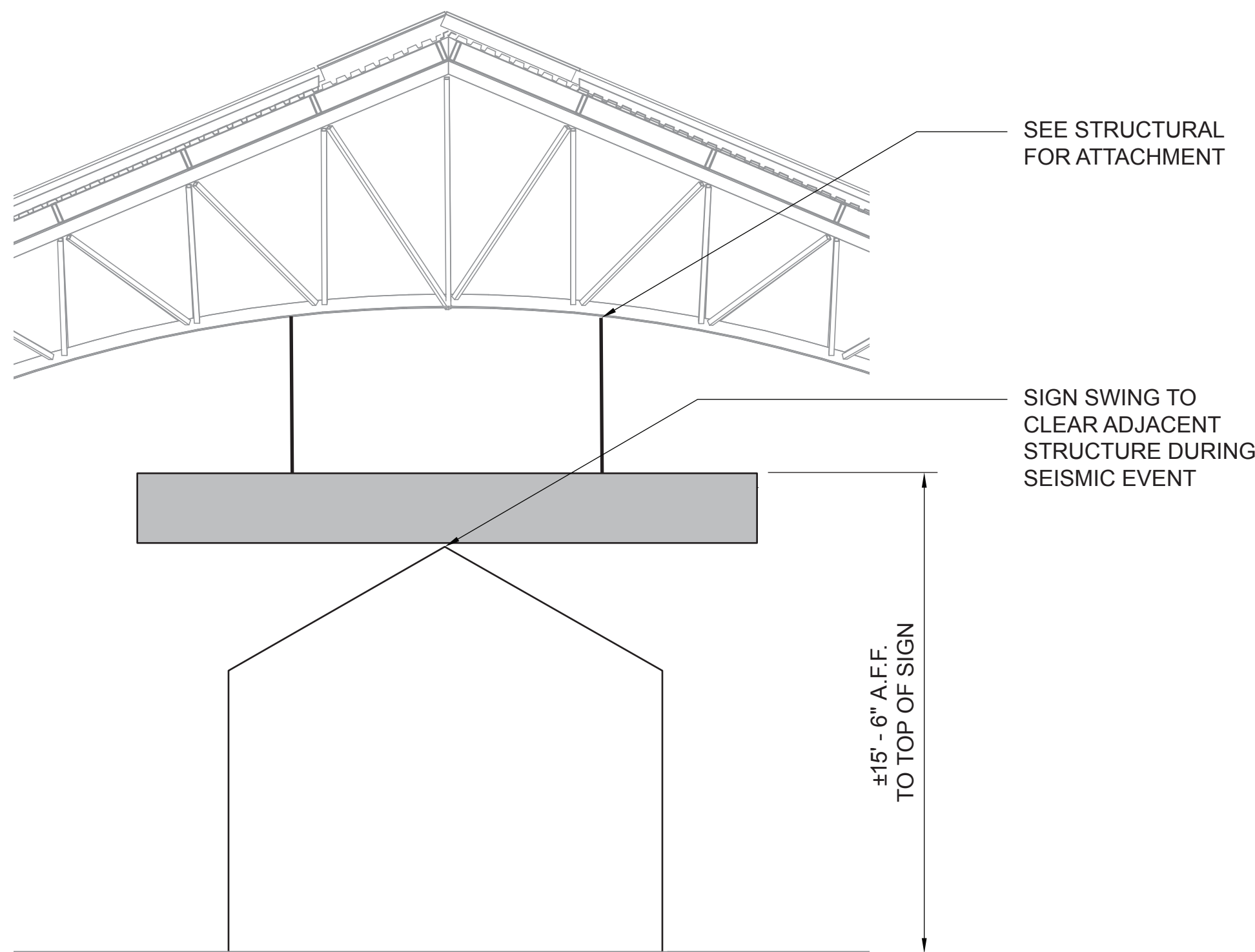
3 CM2 - MOUNTING CONDITION CM2-013 SCALE: 1/4" = 1' - 0"
