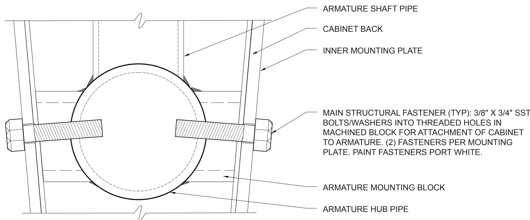
7 CM2 - ARMATURE DETAIL BOTTOM SCALE: FULL SIZE
