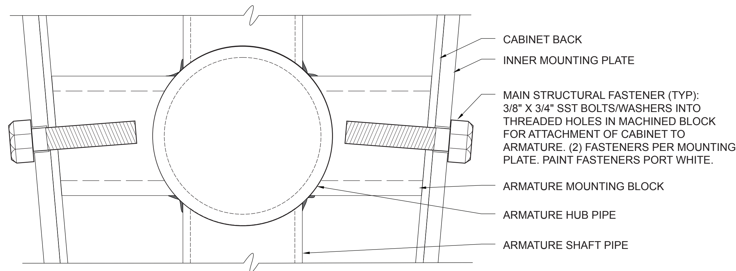
5 CM2 - ARMATURE DETAIL TOP SCALE: FULL SIZE
