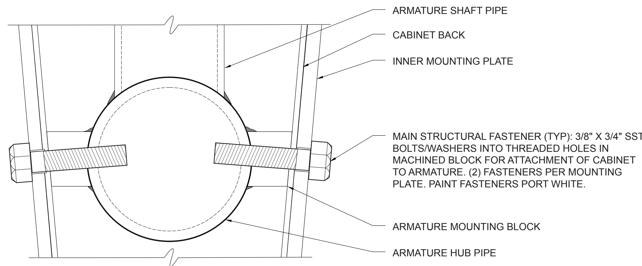
8 CM2 - ARMATURE DETAIL BOTTOM SCALE: FULL SIZE
