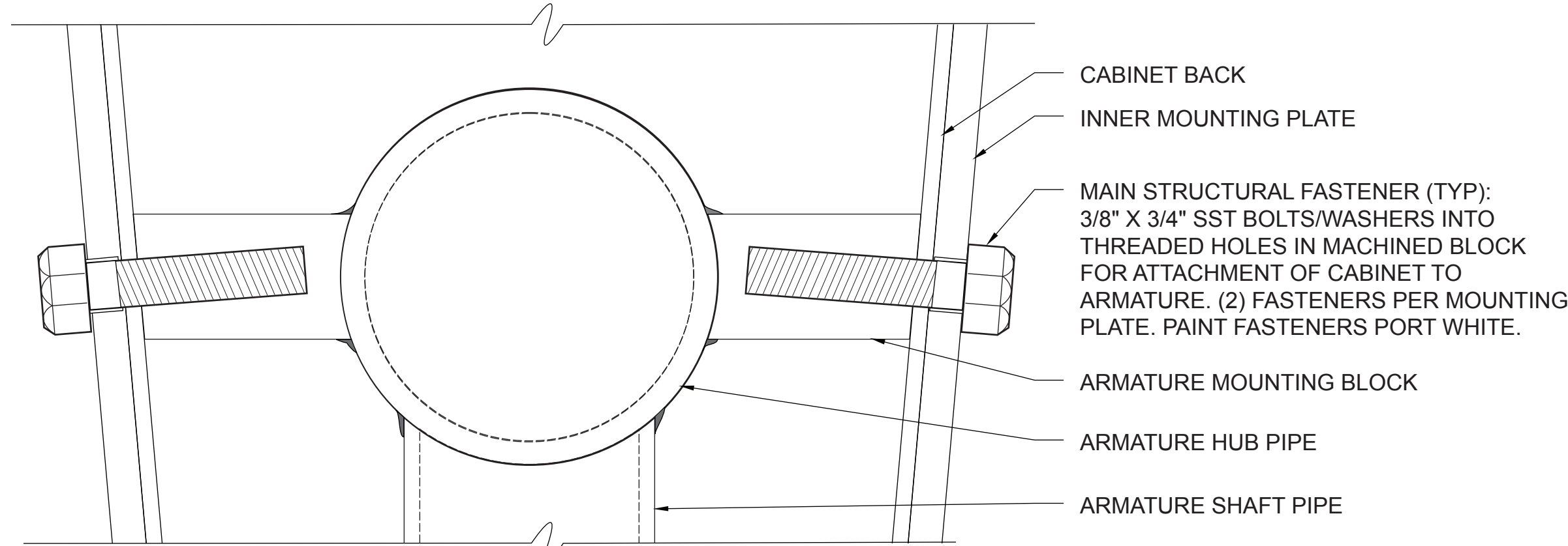
6 CM2 - ARMATURE DETAIL TOP SCALE: FULL SIZE
