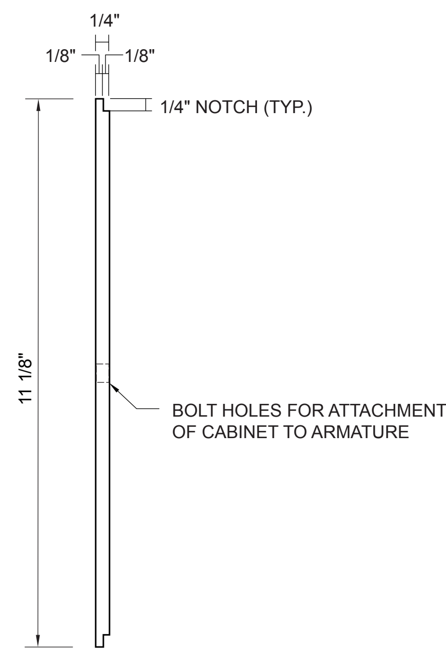
4 CM2 - INNER MOUNTING PLATE SMALL - SECTION SCALE: HALF SCALE
