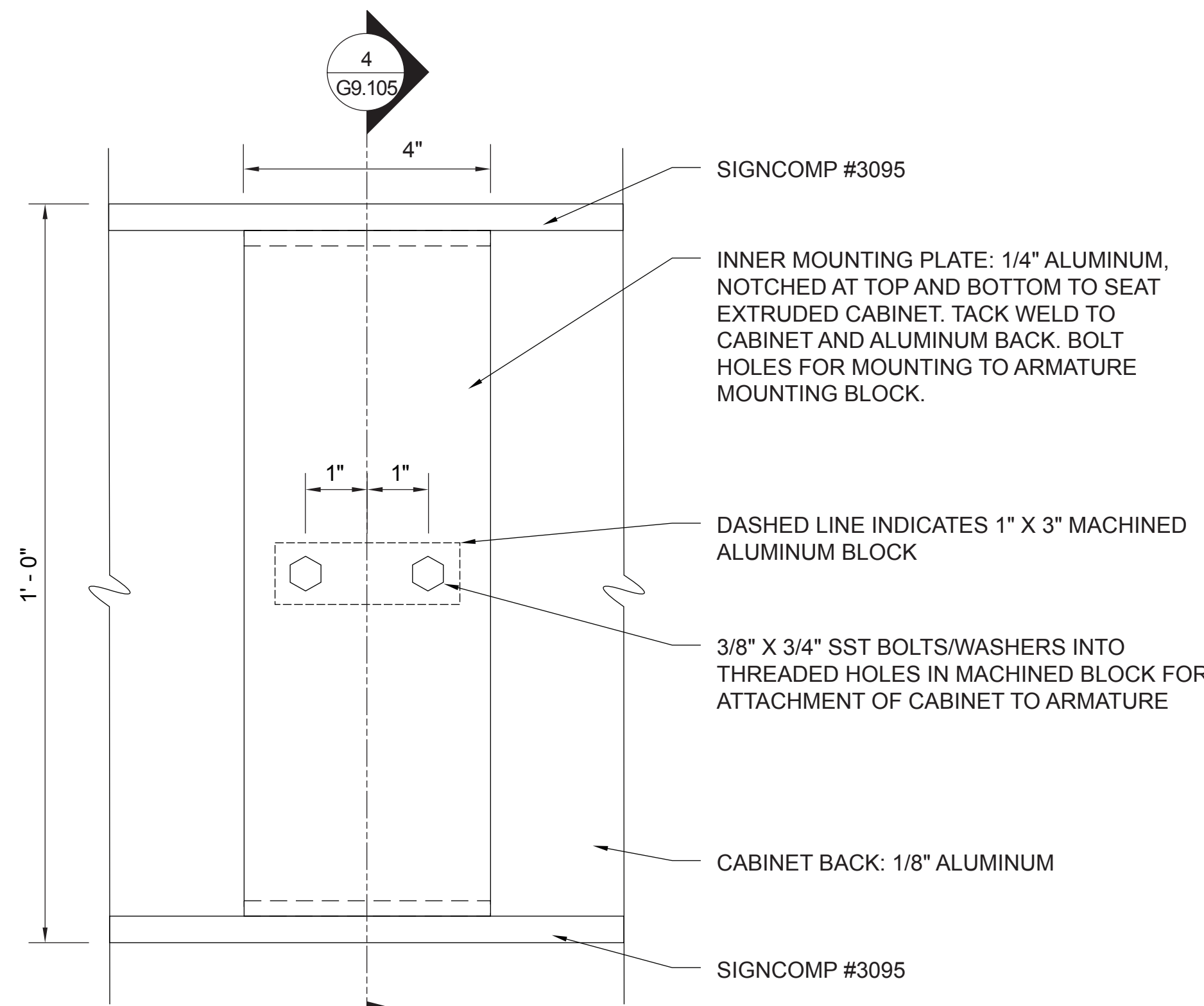
3 CM2 - INNER MOUNTING PLATE SMALL - ELEVATION SCALE: HALF SCALE
