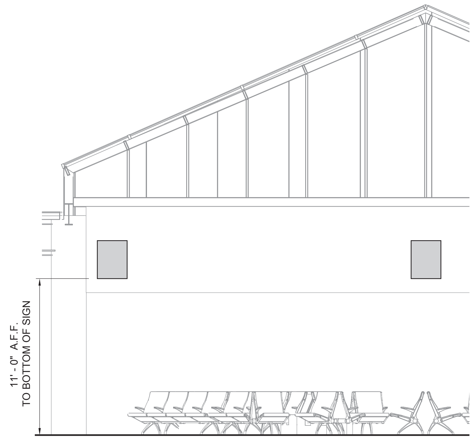
1 WM4 - MOUNTING CONDITION SCALE: 1/4" = 1' - 0"
