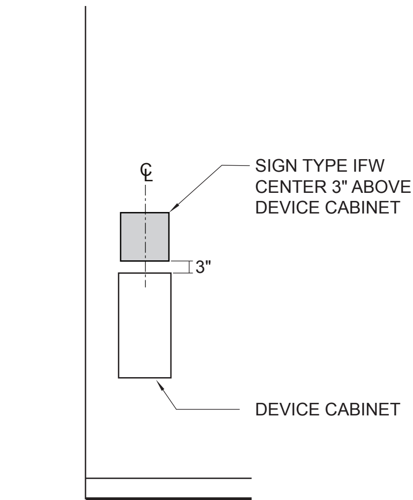
1 IFW - TYP. MOUNTING CONDITION SCALE: 1/2" = 1' - 0"
