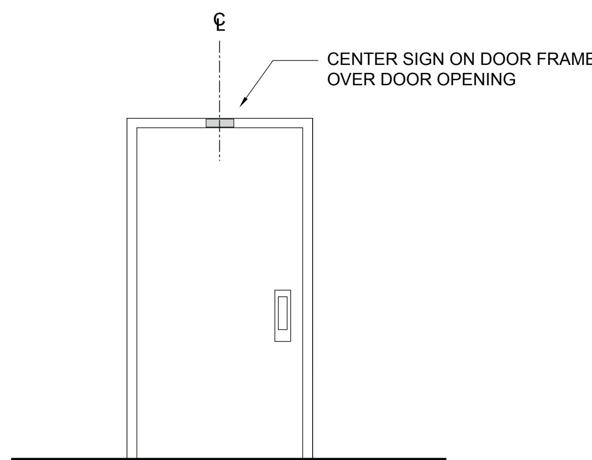
NOTES: 1. SIGN TYPE ID1 CONSISTS OF TWO SIGNS. 2. SIGN NUMBER TAG ON LOCATION PLANS POINTS TO MESSAGE A. MESSAGE B IS A SEPARATE SIGN THAT ATTACHES TO OPPOSITE SIDE OF DOOR. 2 ID1 - TYP. MOUNTING CONDITION @ SINGLE DOOR SCALE: 1/2" = 1' - 0"
