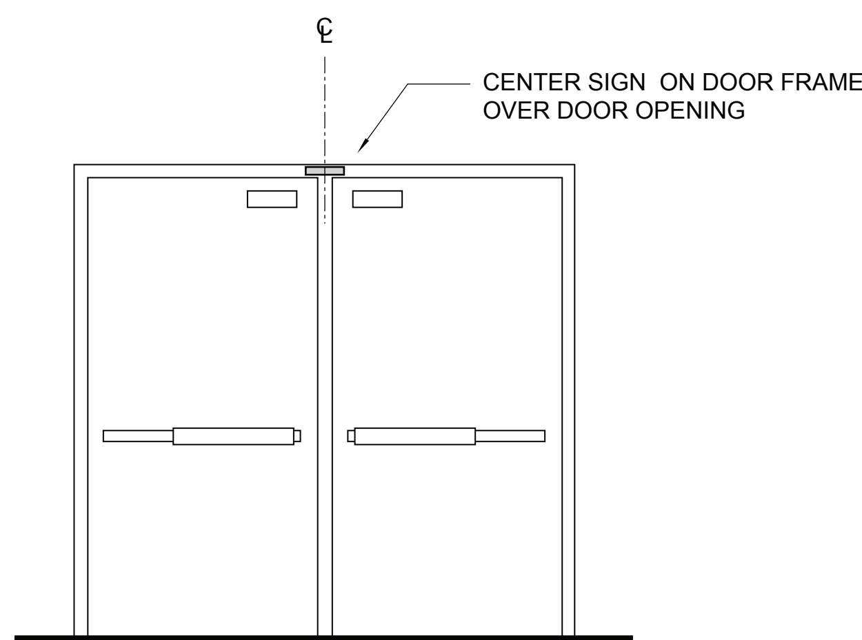
NOTES: 1. SIGN TYPE ID1 CONSISTS OF TWO SIGNS. 2. SIGN NUMBER TAG ON LOCATION PLANS POINTS TO MESSAGE A. MESSAGE B IS A SEPARATE SIGN THAT ATTACHES TO OPPOSITE SIDE OF DOOR. 3 ID1 - TYP. MOUNTING CONDITION @ DOUBLE DOORS SCALE: 1/2" = 1' - 0"
