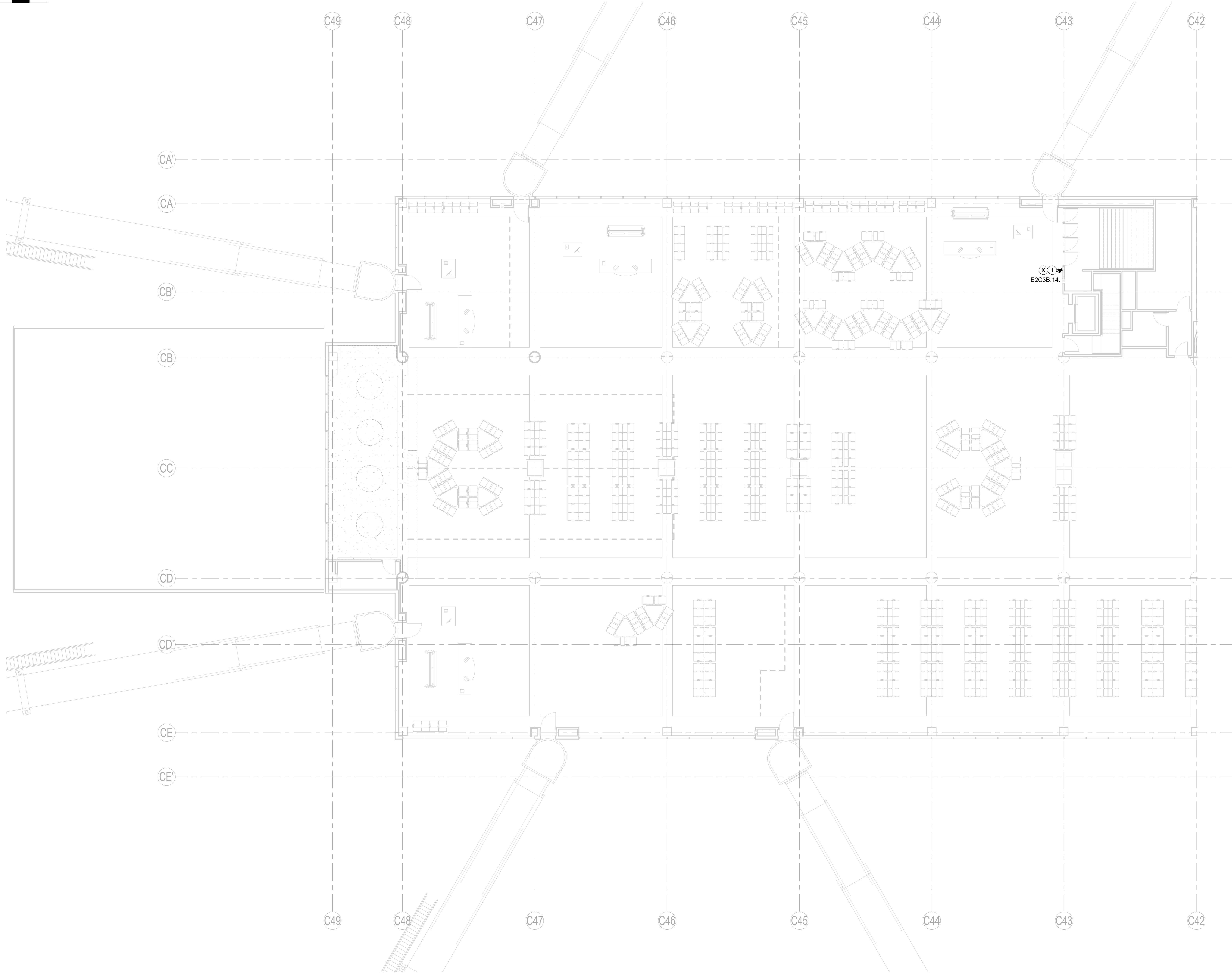
1 CONCURSE C - ENPLANING - SECTOR 70 - DEMOLITION FLOOR PLAN - ELECTRICAL SCALE: 1/8" = 1'-0"
