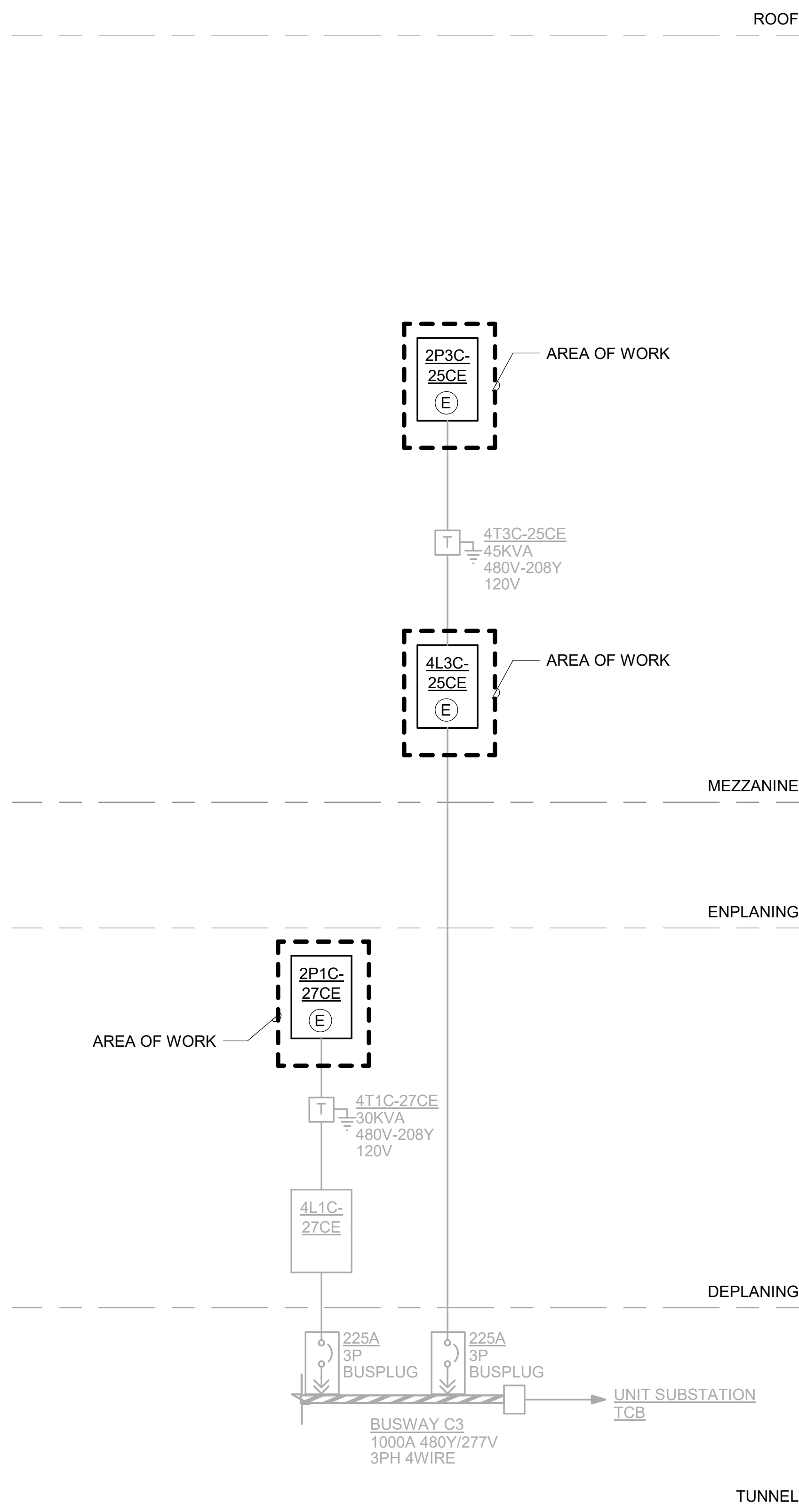
3 PARTIAL ONE LINE DIAGRAM - BUSDUCT C3 SCALE: NONE
