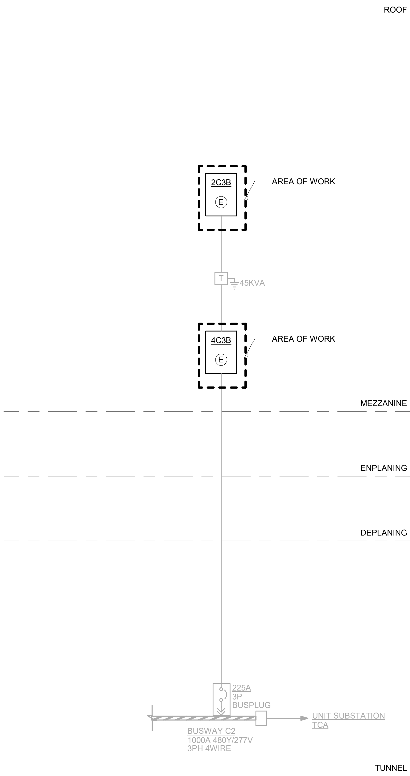
2 PARTIAL ONE LINE DIAGRAM - BUSDUCT C2 SCALE: NONE
